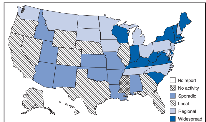
FIGURE 1. Estimated influenza activity levels reported by state epidemiologists, by state and level of activity* — United States, March 26–April 1, 2006
